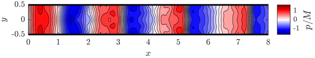
Figure 12: The nonlinear acoustic field within a straight duct, with a perturbation Mach number of M = 0.10 , opening into a duct 10 times larger (outer duct not plotted), in 2D. 10 modes were used in the inner calculation and 200 modes in the outer, with \omega X_1 = 3 for X_1 the inner radius. An animation of this figure is given as Movie 5 in the supplementary material.
