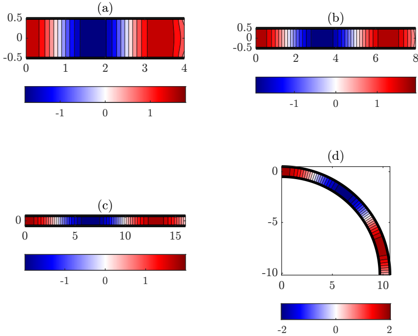
Figure 8: Linear acoustic field within a duct opening into another duct 10 times larger, in 3D, for (a) a straight duct of aspect ratio 1/4; (b) a straight duct of aspect ratio 1/8; (c) a straight duct of aspect ratio 1/16; and (d) a duct of aspect ratio 1/16 undergoing a bend of angle \pi/2 . Each duct has a source at the inlet of frequency equal to that of the duct in question's third closed resonance (as calculated in figure 7). 8 modes were used in the inner duct, 1200 in the outer duct, and the width ratio was 1/40. An animation of this figure is given as Movie 1 in the supplementary material.
