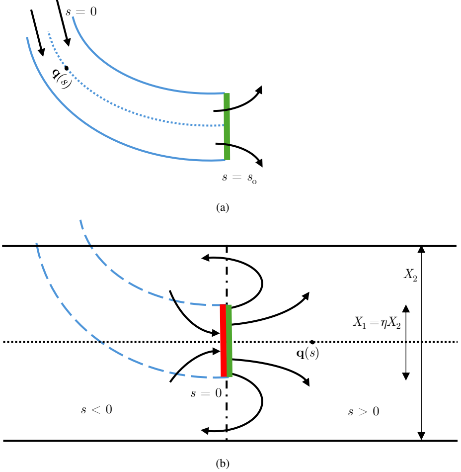
Figure 1: A schematic depicting the inner and outer ducts. (a) The inner duct, with centreline q(s) , inlet ( s = 0 ), and the outlet boundary/surface of emission ( s = s_0 ) depicted in green. (b) The outer duct, with centreline q(s) , relative duct widths X_1 and X_2 , the acoustic source/surface of emission ( s = 0+ ) depicted in green, the absorbing boundary or ‘acoustic wormhole’ ( s = 0- ) depicted in red, and the two domains of propagation s > 0 and s < 0 , with acoustic variables continuous across the dash-dotted line. Note that the outer duct domain s < 0 intersects with the inner duct domain, shown by the blue dashed lines, but this intersection is ignored in this model. Outer and inner widths X_2 and X_1 use the 2D notation.
