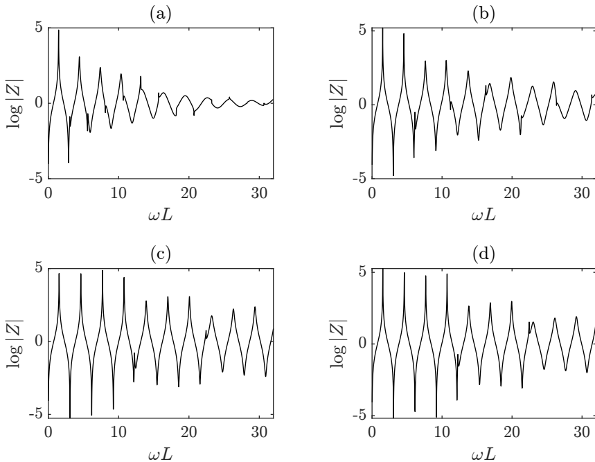
Figure 7: Inlet scalar impedance ( Z_{\text{rms}} in equation 5.1) for a range of frequencies in 3D, for (a) a straight duct of aspect ratio 1/4; (b) a straight duct of aspect ratio 1/8; (c) a straight duct of aspect ratio 1/16; and (d) a duct of aspect ratio 1/16 undergoing a constant-curvature bend of angle \pi/2 . 8 modes were used in the inner duct, 1200 in the outer duct, and the width ratio was 1/40.
