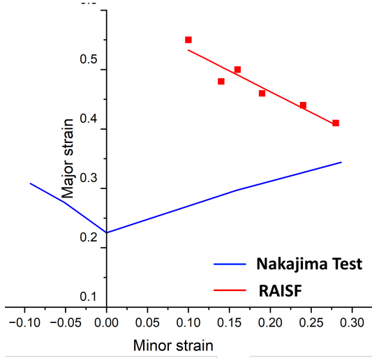
Figure 8: Strains obtained from the RAISF and forming limit curve (FLC) of the material obtained from the Nakajima test.
