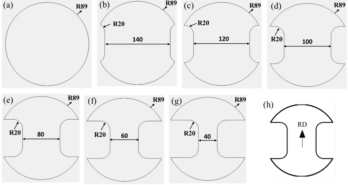
Figure 7: (a-g) Specimen geometries for the generation of FLC and (h) preferred orientation of the specimens used in FLC testing.
