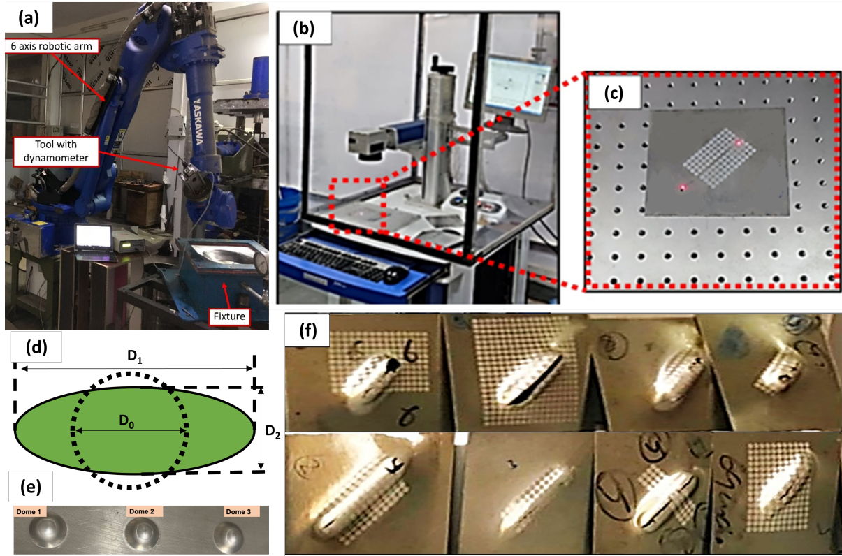
Figure 1: (a) RAISF setup at IIT, Varanasi (b) Laser Engraver for imprinting metallic sheets (c) Sheet Engraved with circular grid pattern (d) Measurement of Ellipse transformed from circle.
