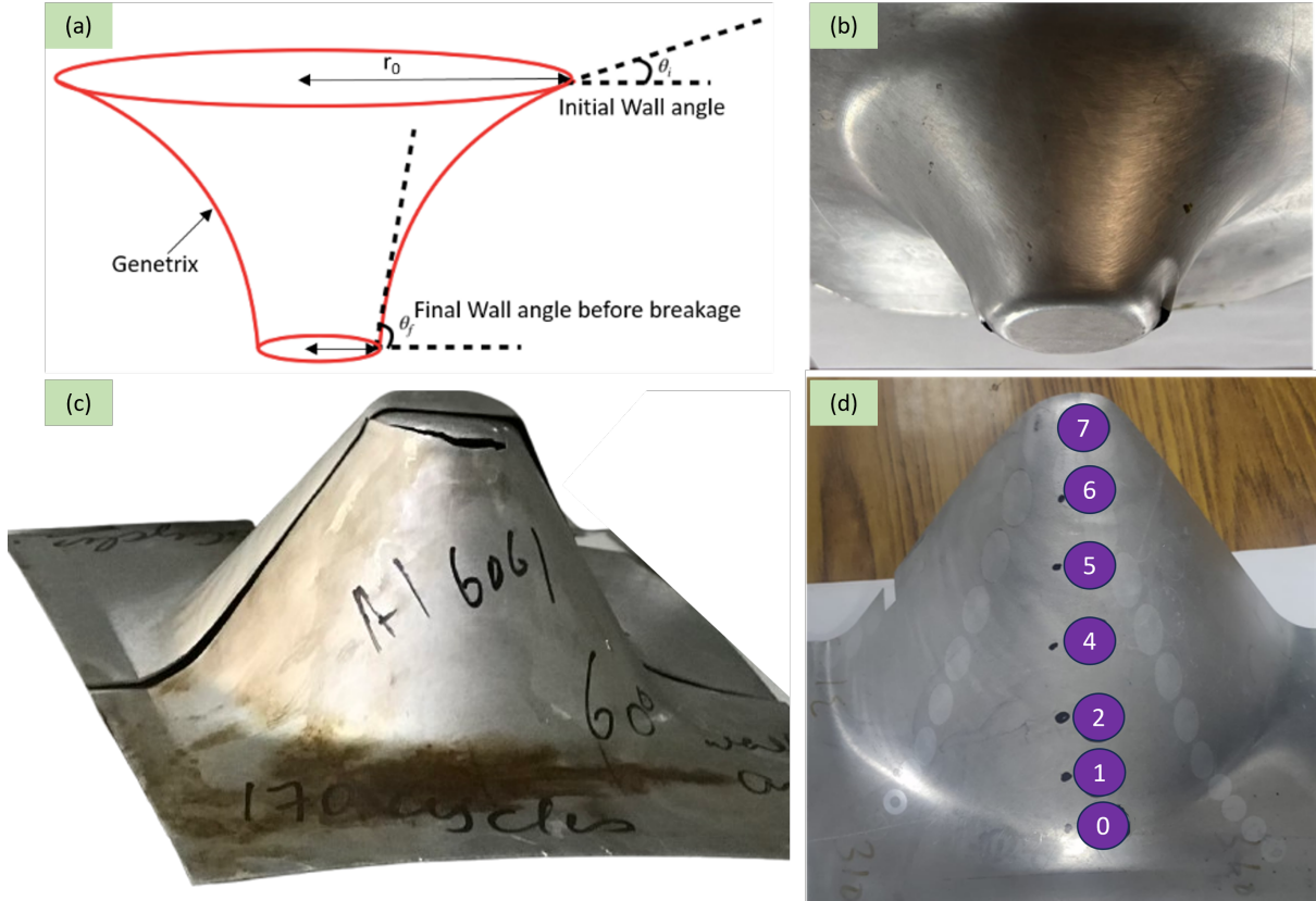
Figure 6: (a) Genetrix of VWACF, (b) fabricated VWACF, (c) fabricated conical frustum of wall angle 600 and (d) cone with circles distorted into ellipses.
