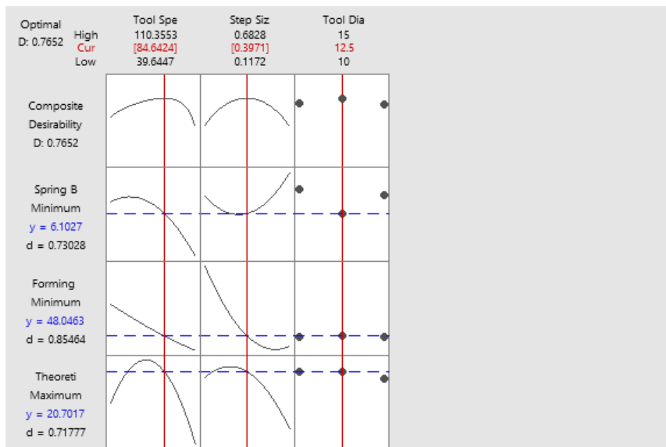
Figure 5: Optimization plot for Tool diameter, Tool speed and step size
