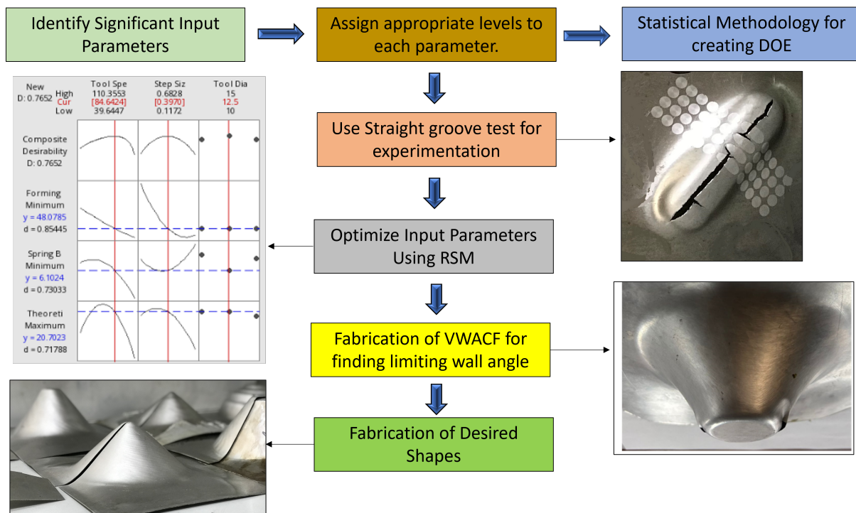
Figure 9: Proposed methodology for formability evaluation in RAISF.
